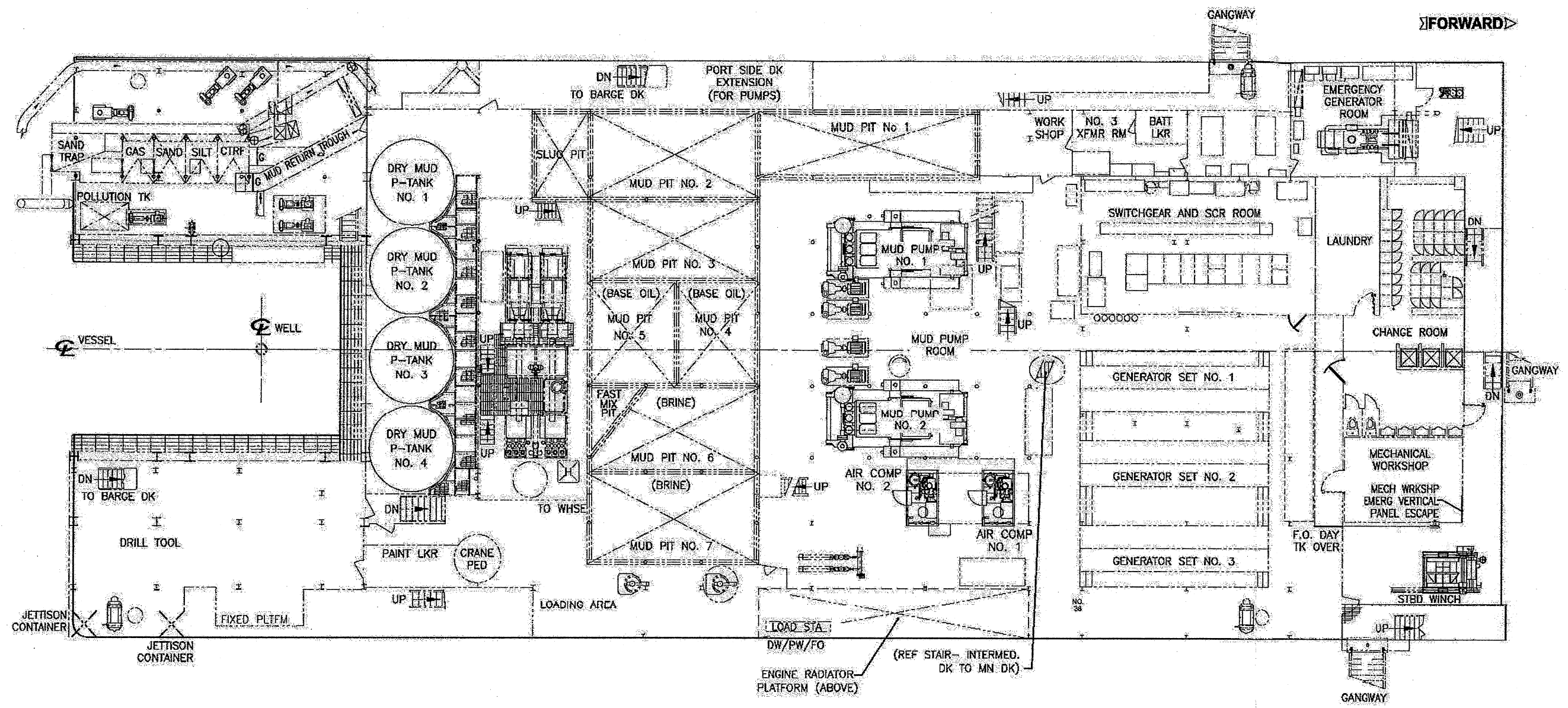
MACHINERY DECK EL: 27'-11 1/2" TOP OF PLATE AT 24'-0" OFF CENTER TO OUTBOARD EDGE (SLOPE 1/4" PER FT. FROM 24'-0" OFF CENTER TOWARDS CENTER OF RIG)
