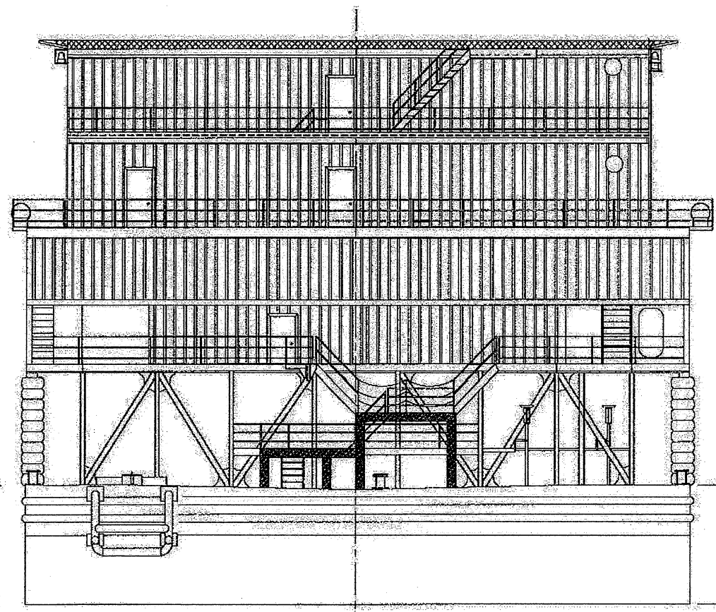
FORWARD END ELEVATION LOOKING AFT.
