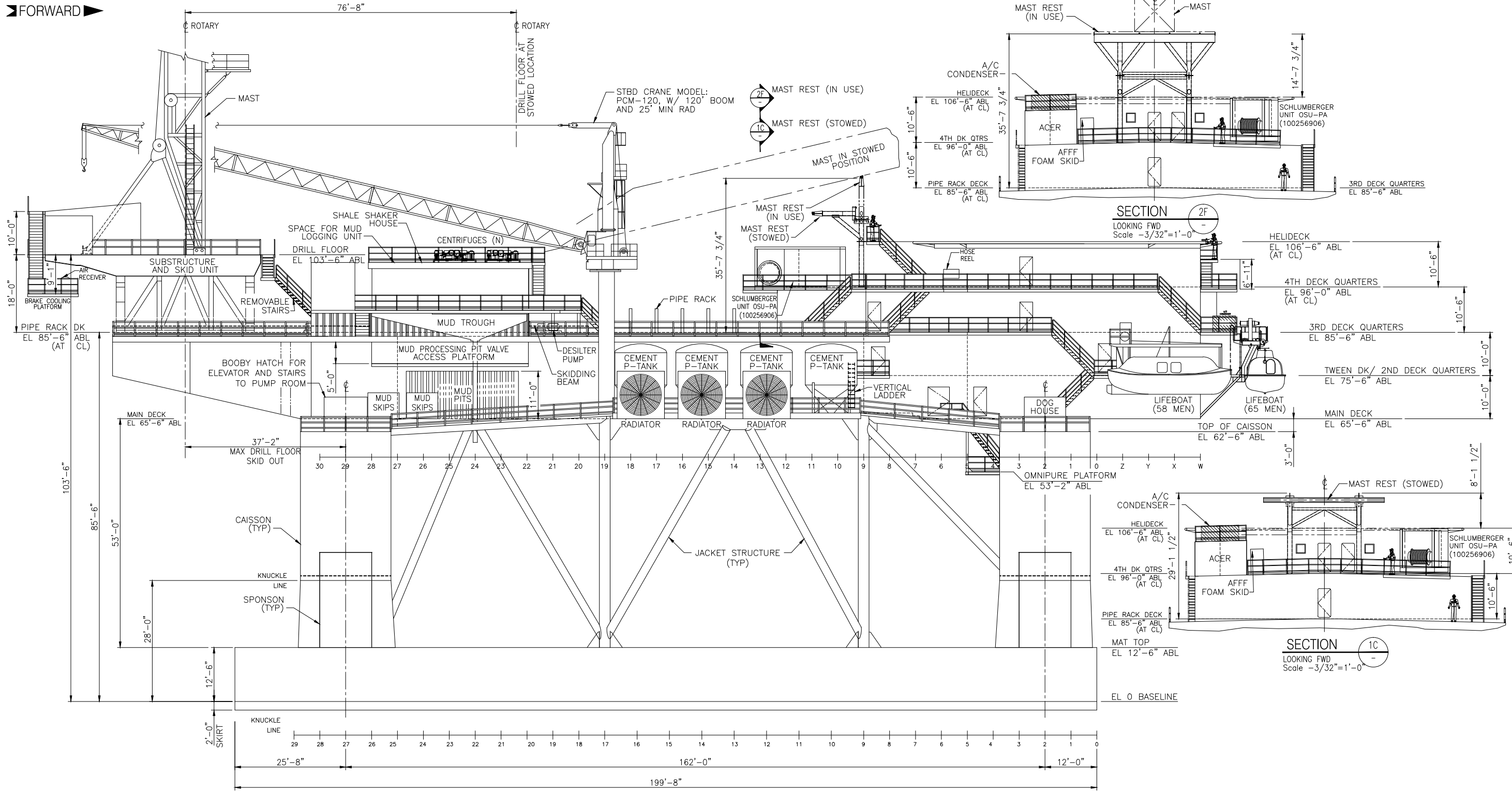
GENERAL ARRANGEMENT STARBOARD OUTBOARD PROFILE
