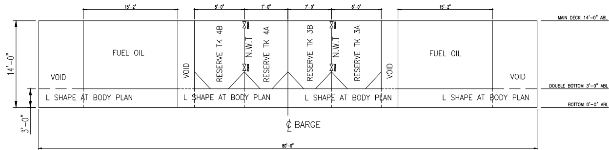
FRONT VIEW @ FR# 15
