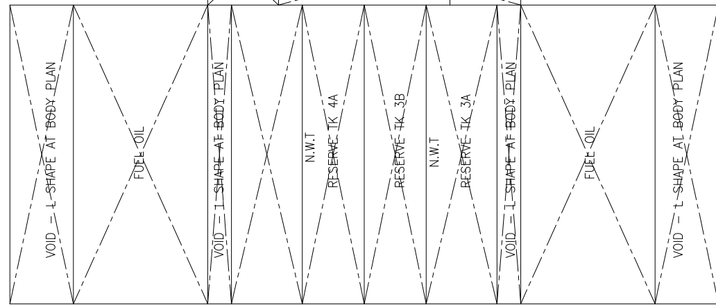
DOUBLE BOTTOM PLAN
