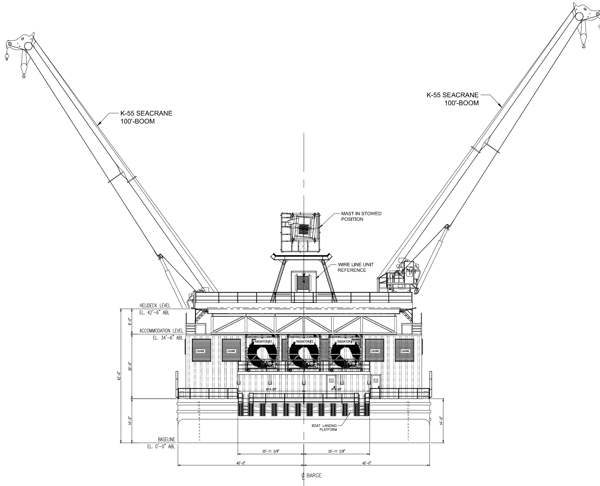
FRONT VIEW
