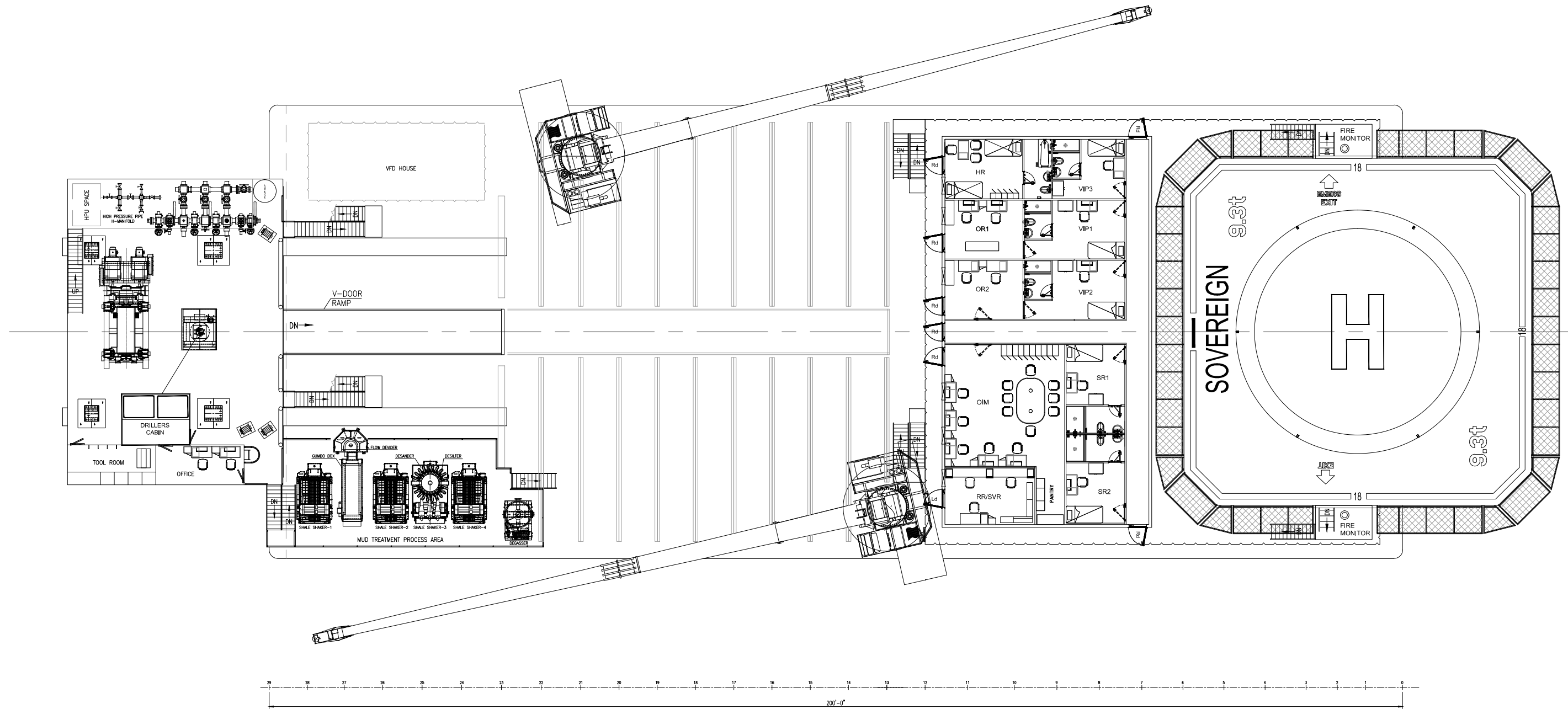
DRILL FLOOR AND HELIDECK PLAN VIEW EL. 44'-0" ABL
