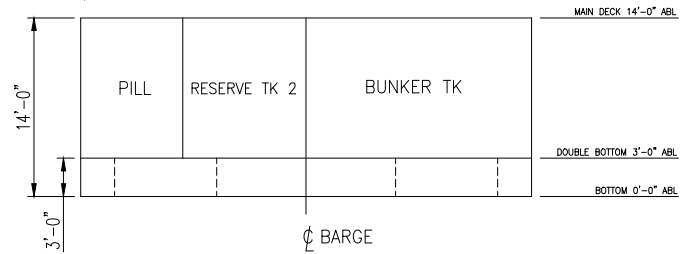
FRONT VIEW @ FR # 20
