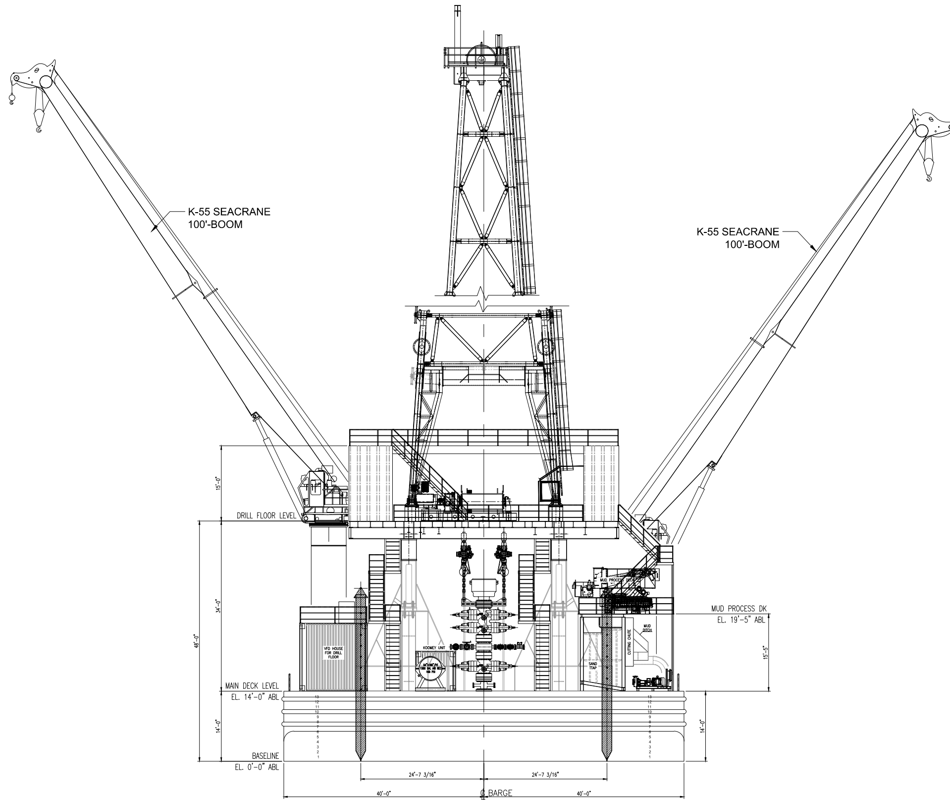
AFT VIEW
