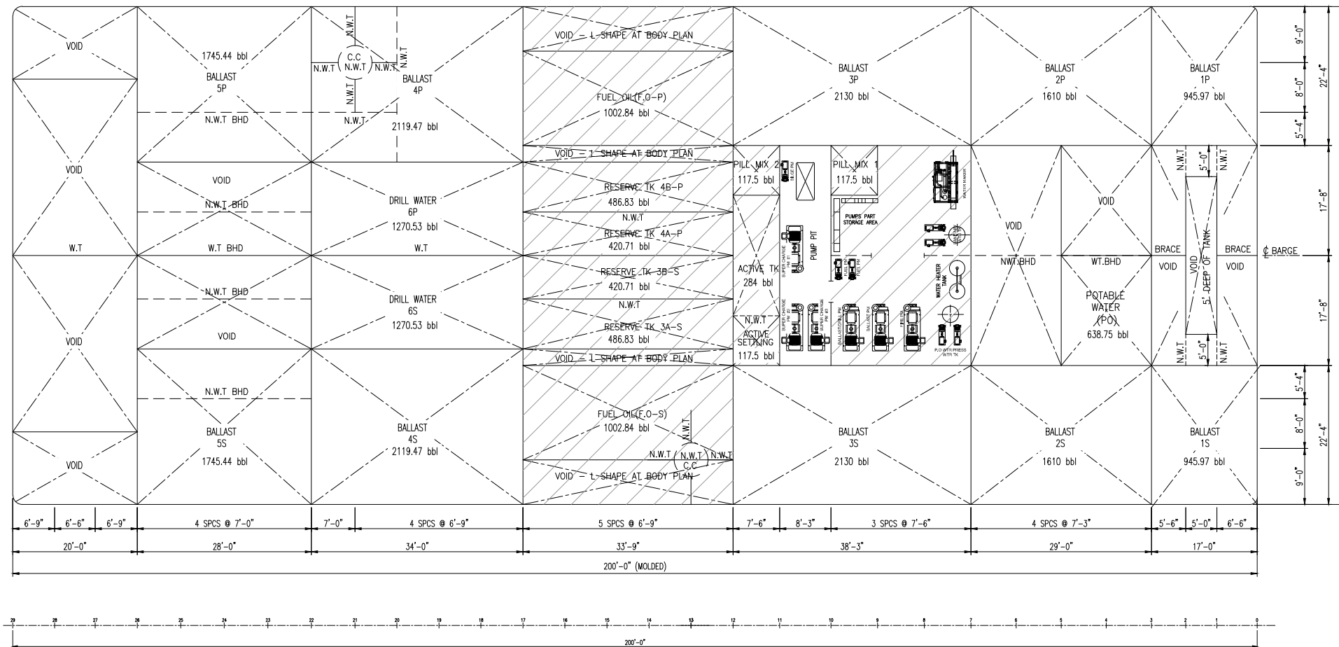
BARGE DECK TANK PLAN PLAN VIEW
