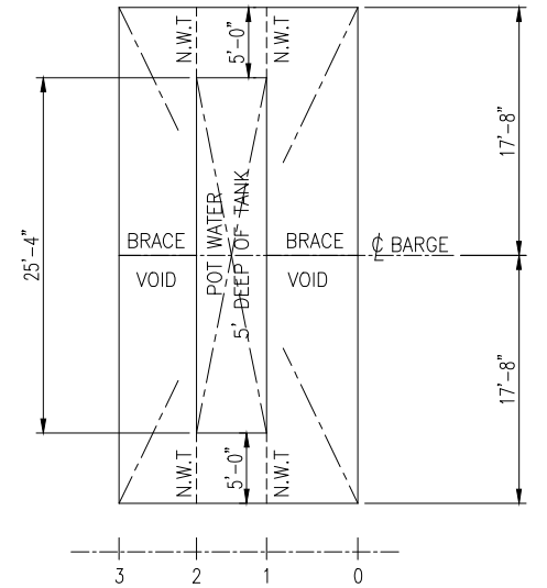
MAIN DECK PLAN
