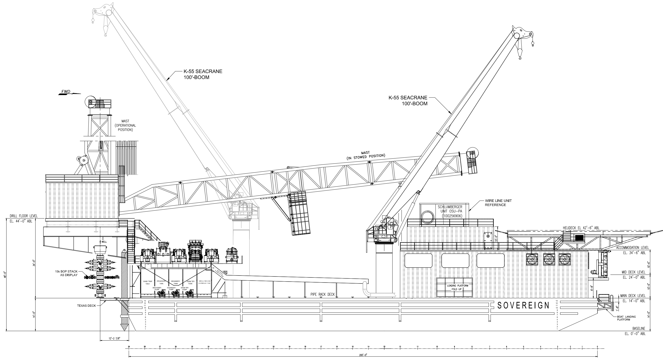
STARBOARD PROFILE
