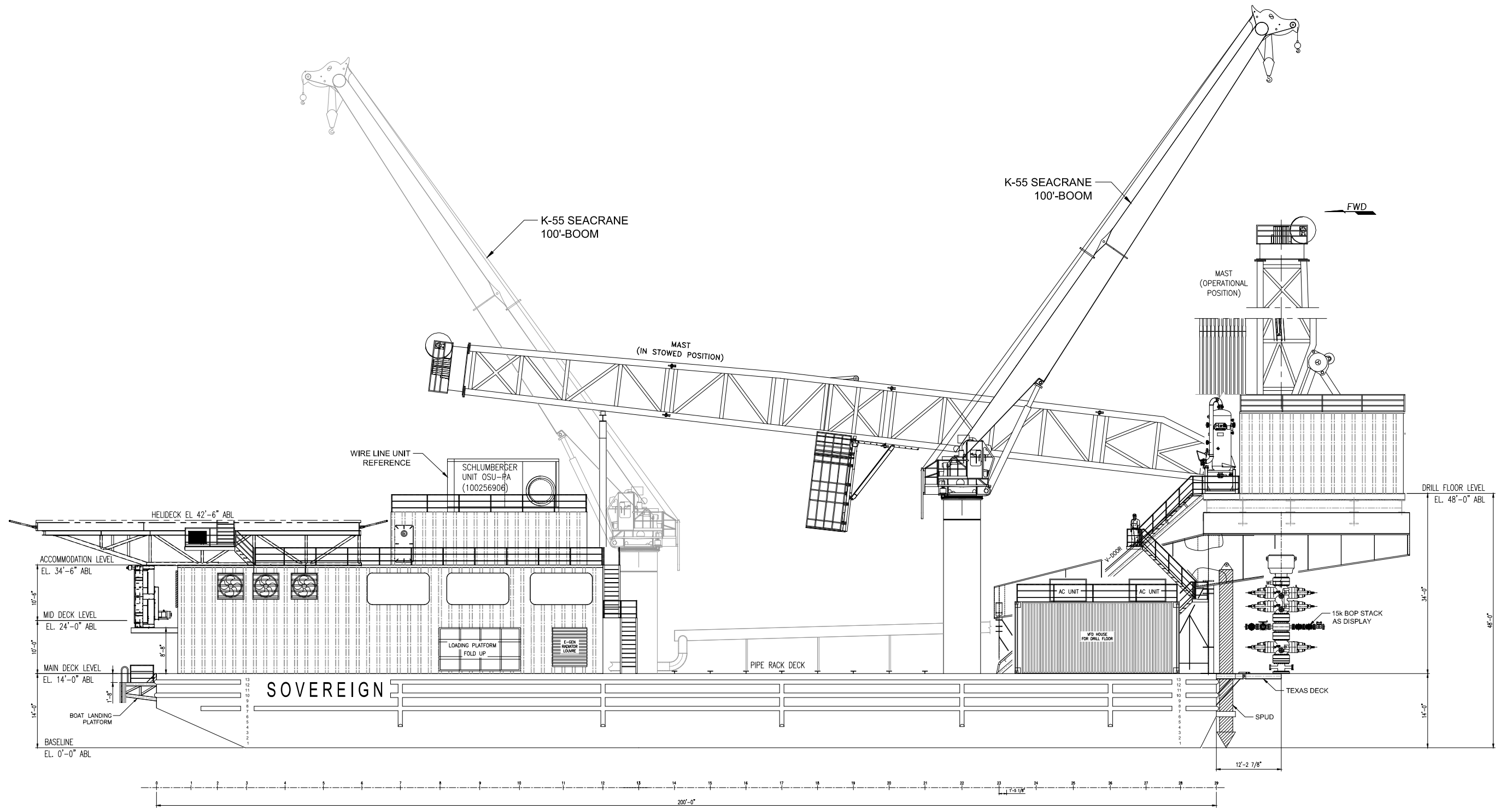
PORT PROFILE
