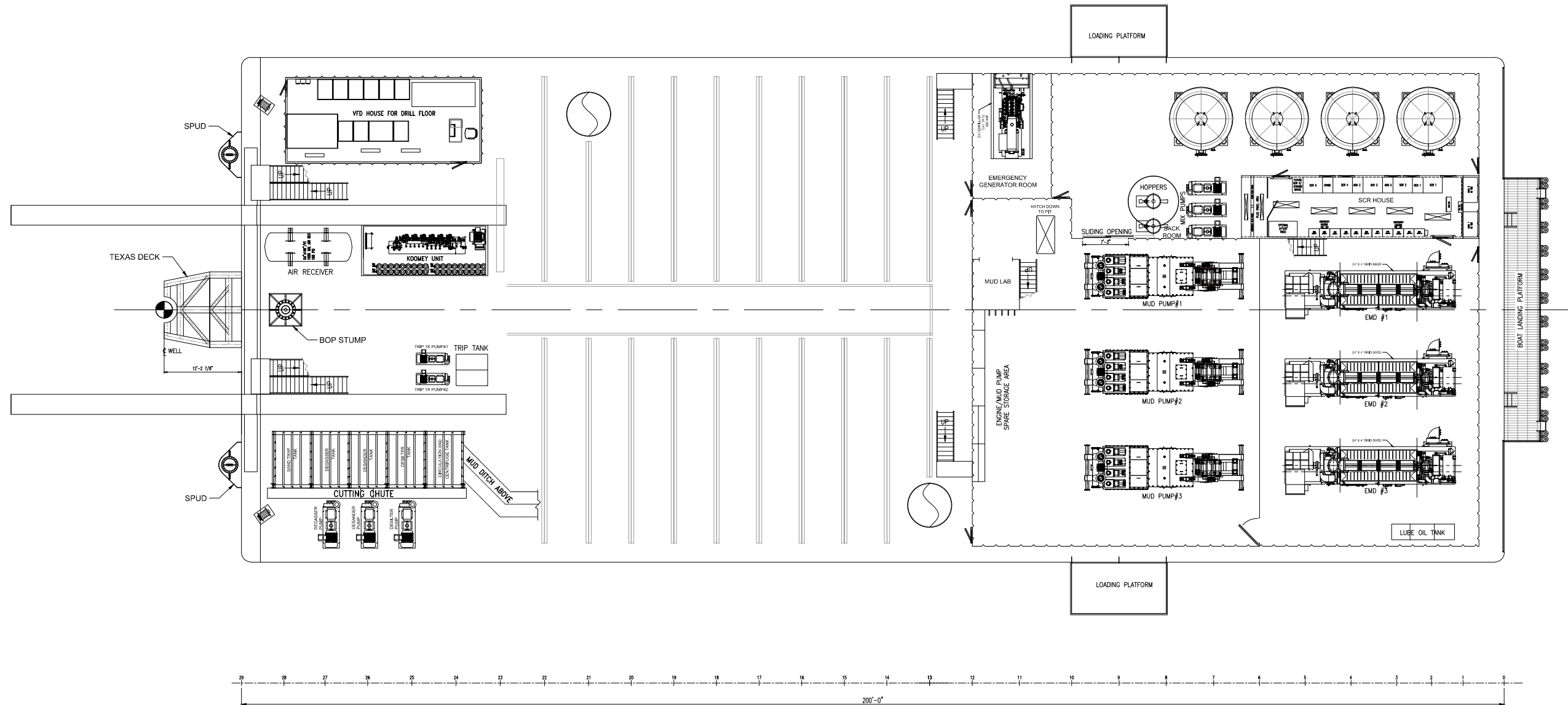
MAIN DECK PLAN EL. 14'-0" ABL
